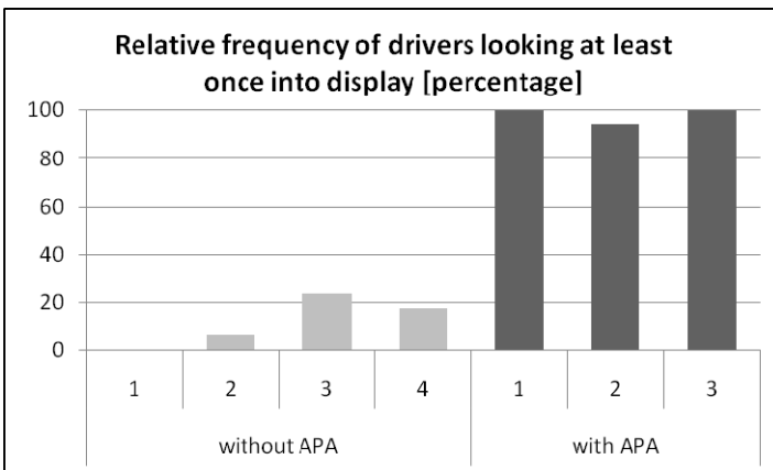
Fig.7. Relative frequency of drivers who look at least once into the system’s display [in percentage] during the first parking motion with and without the APA system, respectively
