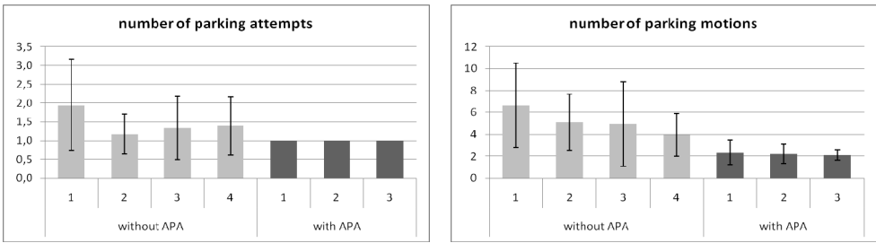
Fig.2. Mean number of parking attempts (left) and mean number of parking motions (right).
